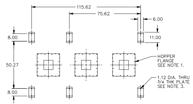
ANCHOR BOLT PLAN
