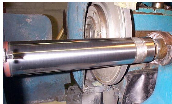
Forklift truck hydraulic ram, previously hard chromed, now coated with JK ® 120H. As sprayed (left) and during surface finishing (right) to 7 μ-inches (0.018μm).
