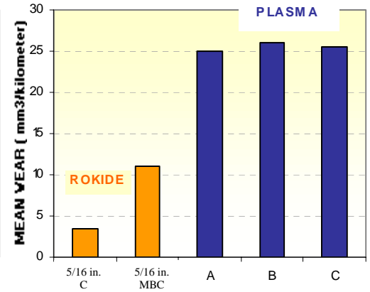
Dry Abrasion Wear (ASTM G65) of ROKIDE and Plasma Chrome Oxide Coating
