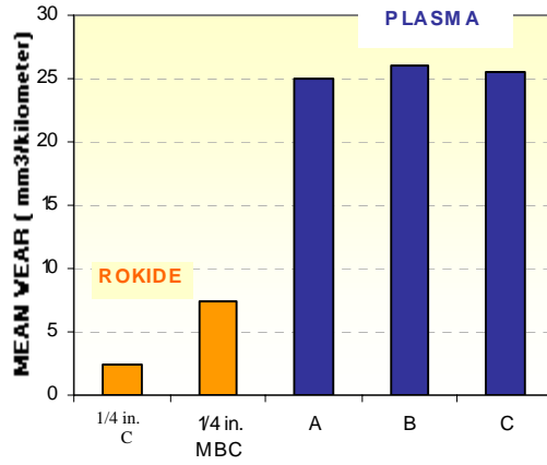
Dry Abrasion Wear (ASTM G65) of ROKIDE and Plasma Chrome Oxide Coating
